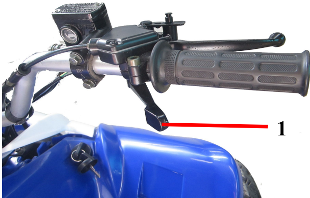
1. Throttle lever
