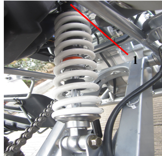
1. Spring preload adjusting ring
