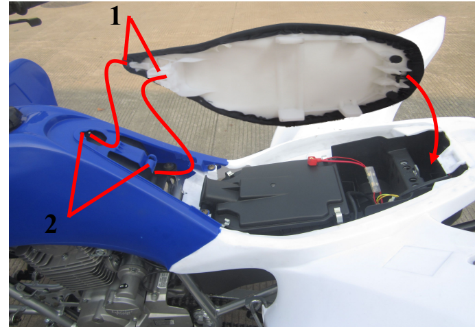
1. Projection 2. Seat holder
